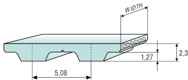
TOOTH PROFILE ACCORDING TO ISO 5296-1
